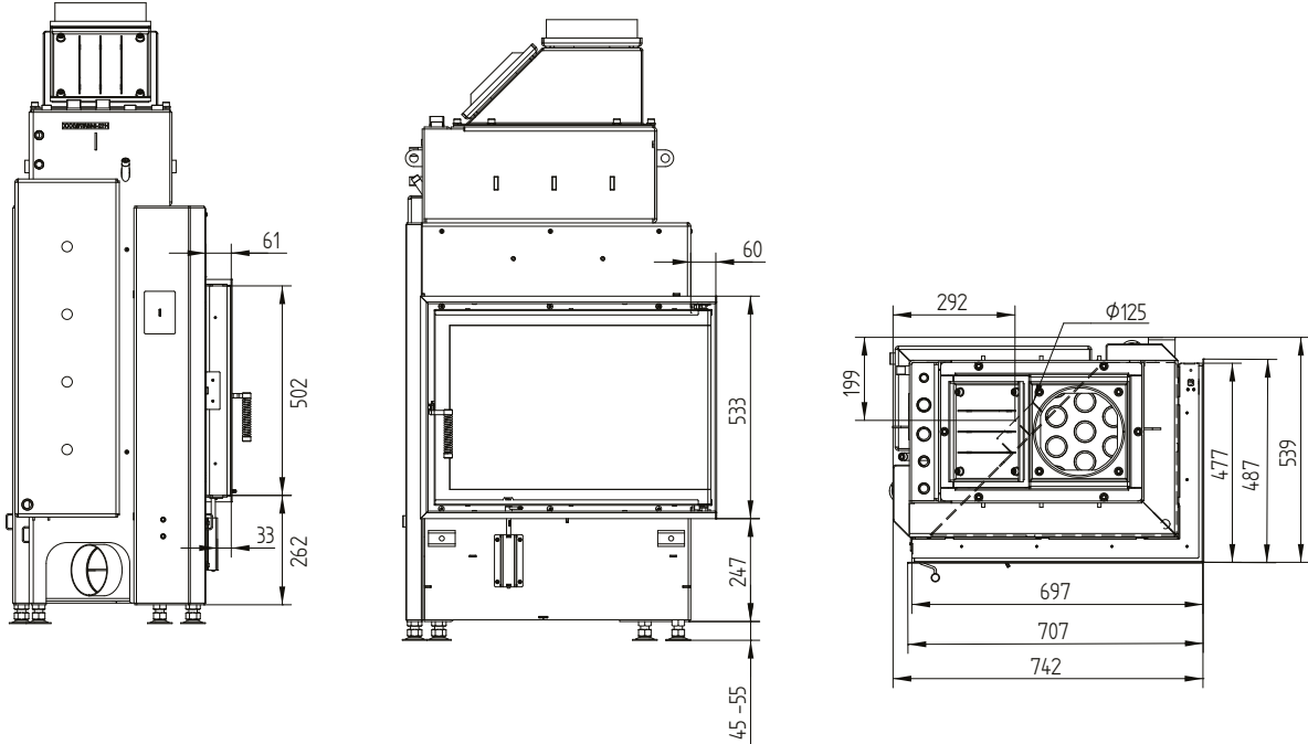
Build-on frame 67/45/51R right side opening 6sides 80 mm / feet
